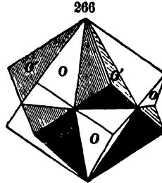
Fluorite.
